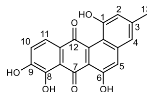
6,9-Dihydroxytetrangulol (6,9-DHT)
